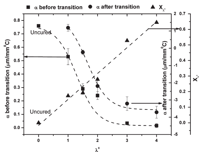
Figure 22. \alpha of SBS competitive double network elastomers before and after the transition point with increase in extent of cure ( X_{\lambda^c}^c ) at various \lambda^c .
