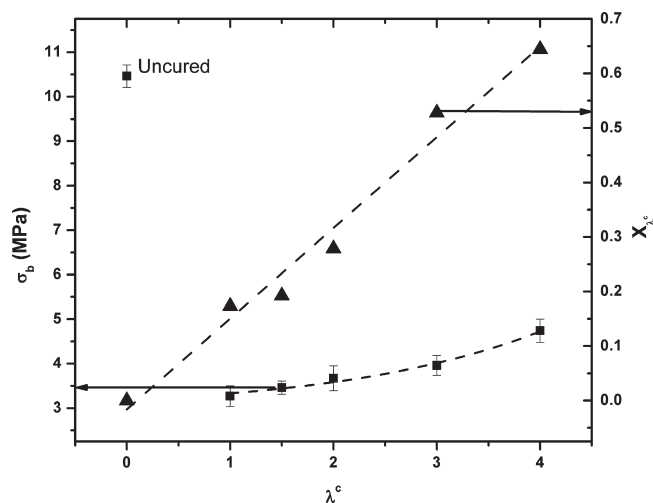
Figure 7. Increase in \sigma_b with increase in extent of cure during stretch ( \chi_{\lambda^c} ) with increase in \lambda^c .
