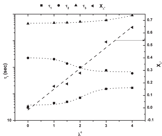
Figure 17. Time constants \tau_1 , \tau_2 , and \tau_3 as a function of \lambda^c and their relationship with extent of cure during stretch ( X_{\lambda^c} ) in high strain regime.
