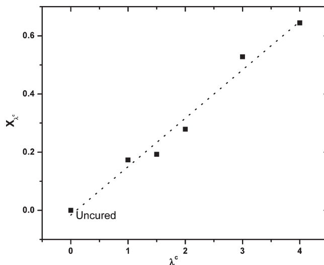
Figure 5. Increase in effective extent of cure during stretch ( X_{\lambda^c}^c ) with increase in \lambda^c .
