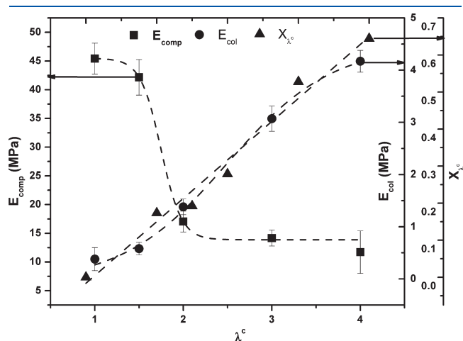
Figure 9. Modulus in low strain ( E_{\text{comp}} ) and high strain ( E_{\text{col}} ) regimes along with increase in extent of cure during stretch ( X_{\lambda^c} ) with increasing \lambda^c .
