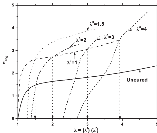
Figure 8. Plot of \sigma_{\text{eng}} vs apparent \lambda , indicating the transition points in the double network elastomers.
