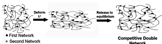
Figure 2. Formation of prestressed competitive double network elastomer.
